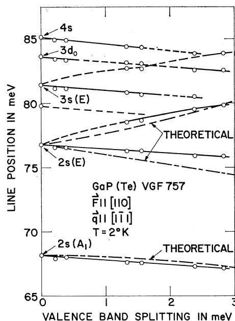
FIG. 4. Stress dependence of the two-electron transition lines observed in photoluminescence. The line positions are measured with respect to the low-energy component of the zero-phonon recombination line of excitons bound to neutral Te donors in GaP. This energy should correspond to the energy involved in the excitation 1s(A_1) \rightarrow ns . The line positions are plotted against valence-band splitting: a parameter linear in stress magnitude with an estimated correspondence of (\Delta_{VB} = 1 \text{ meV}) = 0.27 \times 10^9 \text{ dyn/cm}^2 . The polarization of the photoluminescence was not measured; however, the spectrograph would have been more sensitive to light polarized with the electric vector perpendicular to the stress direction versus parallel to the stress direction by a factor of about 1.5.
